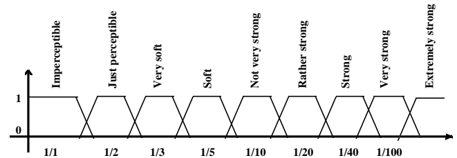
Figure 1 Contrasts presented as fuzzy sets
